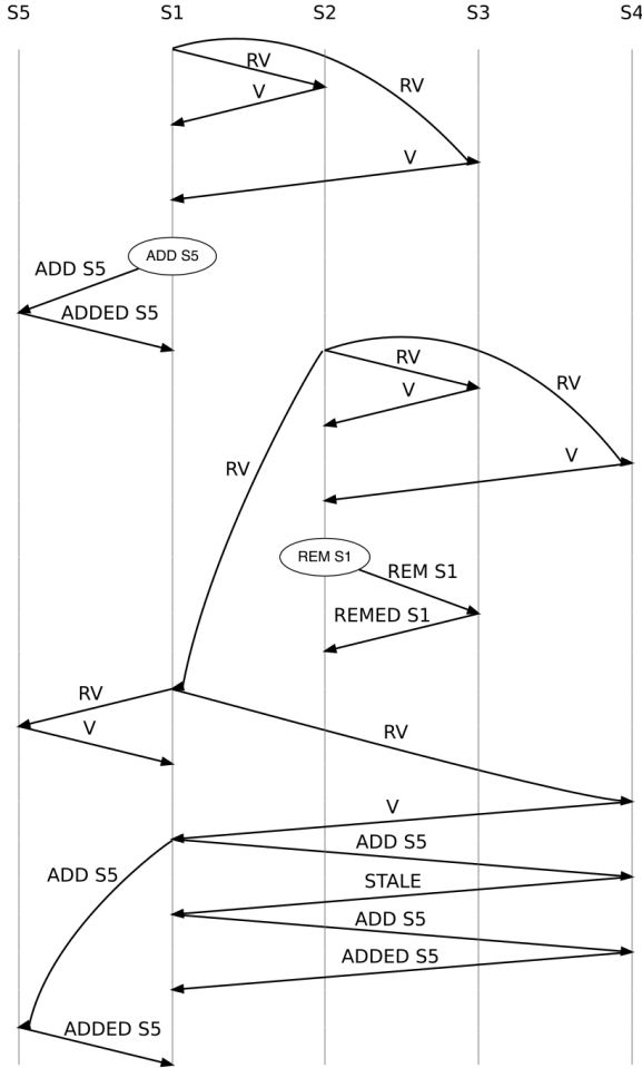
Figure 1: A space-time diagram, generated with Oddity and lightly edited for clarity, illustrating a Raft execution leading to the reconfiguration bug. Each vertical line represents in a node in the system, and arrows between them represent messages. The circles represent messages received from clients of the system (elided for presentation).
