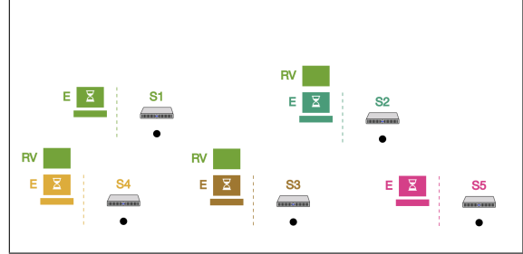
Figure 3: The state of the Raft system in Oddity after S_1 starts an election. S_2 , S_3 , and S_4 have RV messages in their inboxes. The messages have the same color as their sender ( S_1 ).
