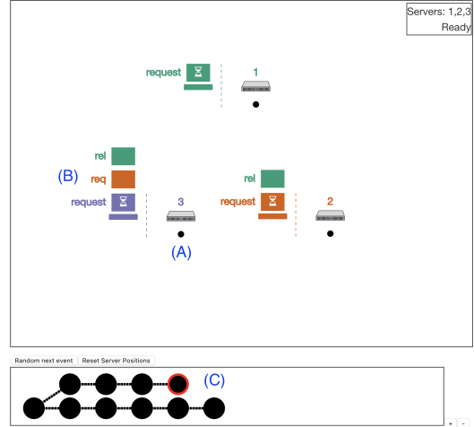
Figure 6: The debugger window. Each node (A) is displayed, along with an inbox (B) of messages and timeouts waiting to be delivered at that node. The user can control delivery by clicking on timeouts and messages, and can also inspect the contents of any message or timeout or the state at any node. Using the branching history view (C), the user can navigate the states of the system they have explored. The user can reset the debugger to a previous state by clicking on it; this resets the system to that state so that the user can explore further from there.
