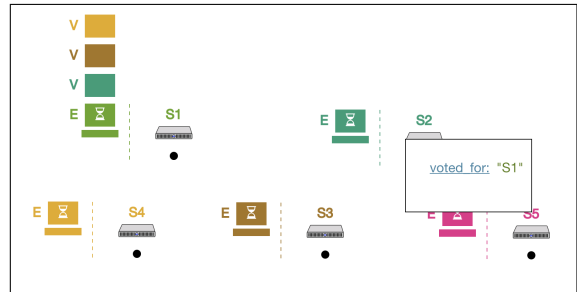
Figure 4: The state of the Raft system in Oddity after S_2 , S_3 , and S_4 respond to S_1 's vote request. The votes from those nodes are in S_1 's inbox, with colors corresponding to the sending node. The engineer has clicked on S_2 to expand its state, showing that it has recorded a vote for S_1 (the Raft protocol requires that nodes track which node they voted for in the current term).
