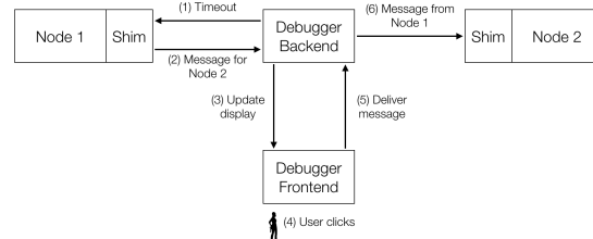
Figure 8: An example of DVIZ components communicating to deliver a message. When Node 1 receives a timeout, either from log replay or user action, it produces a message for Node 2. This message is sent to the debugger backend, which tells the frontend to display it in Node 2’s inbox. When the user clicks the message (which they could do immediately or after delivering other messages and timeouts) the frontend notifies the backend, which sends the message to Node 2.
