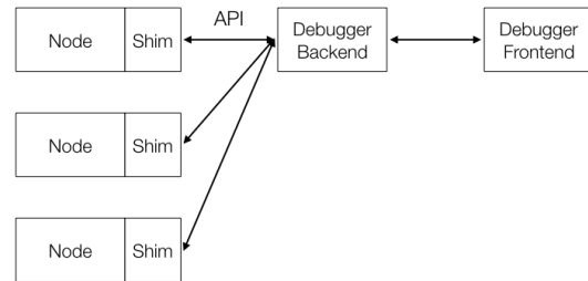
Figure 7: The architecture of the debugger implementation. The debugger backend communicates with individual nodes (each of which has a stub implementing the Oddity API). The debugger frontend, running in the browser, communicates with the backend. Most of the logic runs in the browser, allowing the backend to serve as a thin communication layer.
